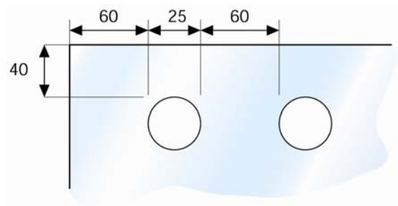
Glass thickness 19 mm
