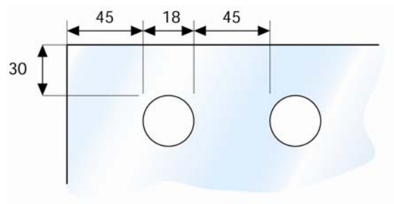
Glass thickness 15 mm
