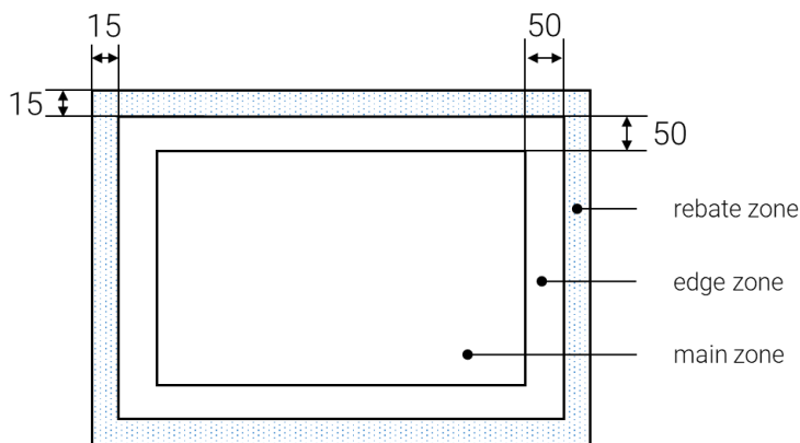
Picture 28: zones for the assessment of visual quality according to ÖNORM EN 1279-1 (dimensions in mm)
