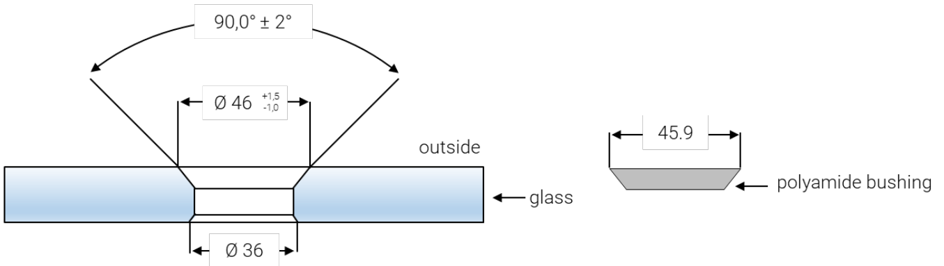
countersunk hole nominal dimensions and tolerances
