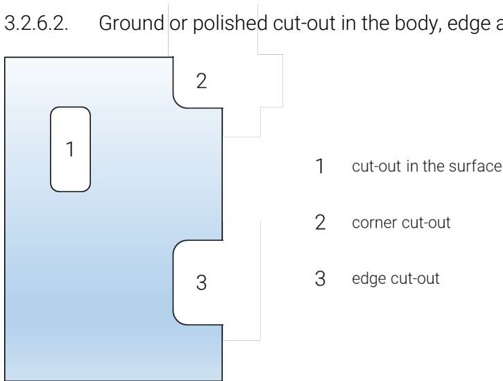
Picture 12: different types of cut-outs
